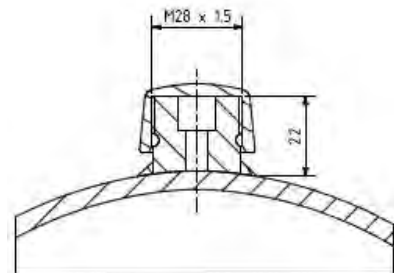
Gas Valve
